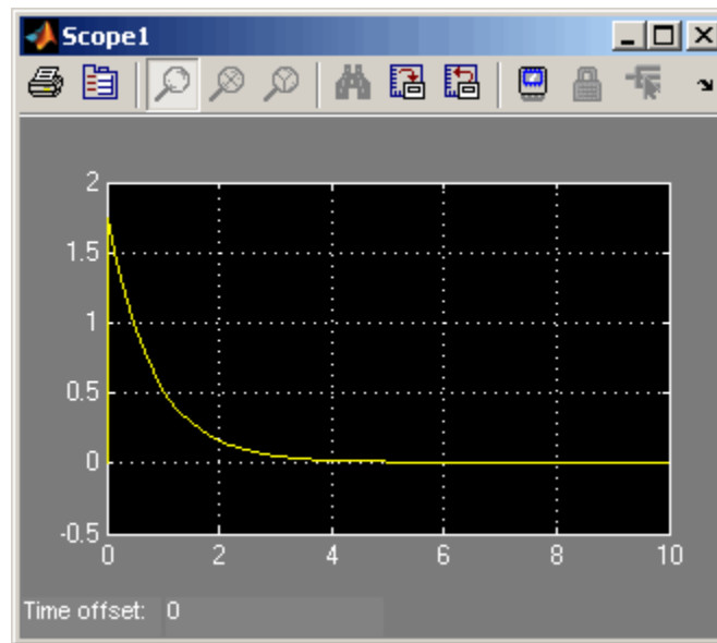
Motor Current
